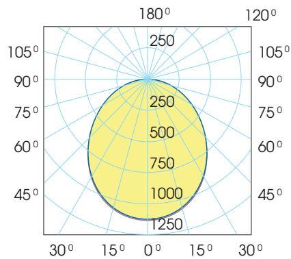
LN08/09 30W
