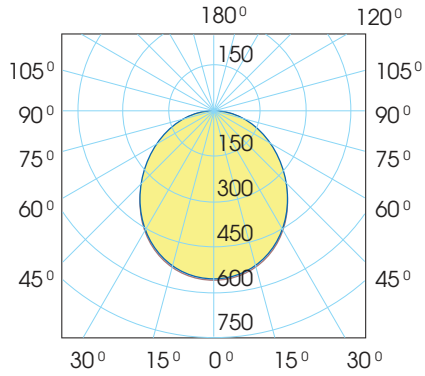
LN08/09 15W
