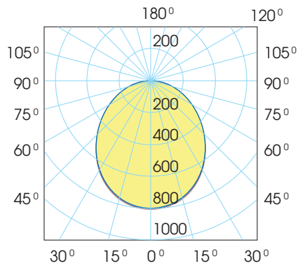
LN08/09 22W
